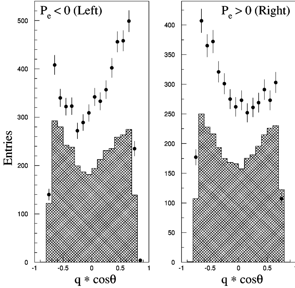
FIG. 7. The distributions of q \cdot \cos \theta_D for the selected D^{*+} meson sample for (a) left- and (b) right-handed electron beams. The solid circles are experimental data, and hatched histograms are RCBG estimated from side-band regions.
